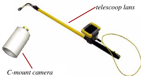
Infrarood camera
